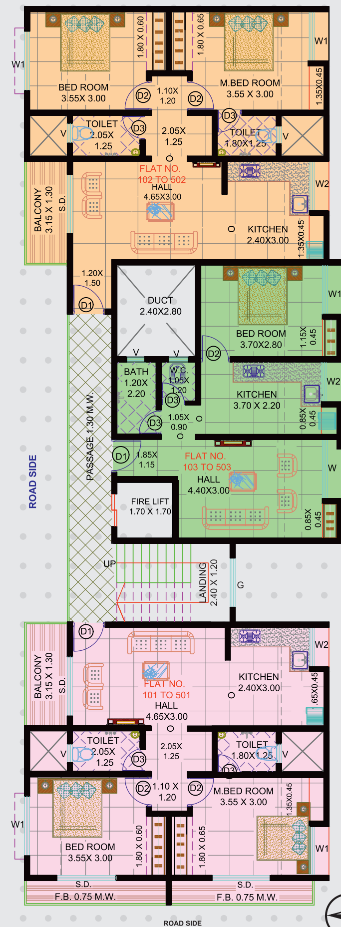
1st to 5th Floor Plan
