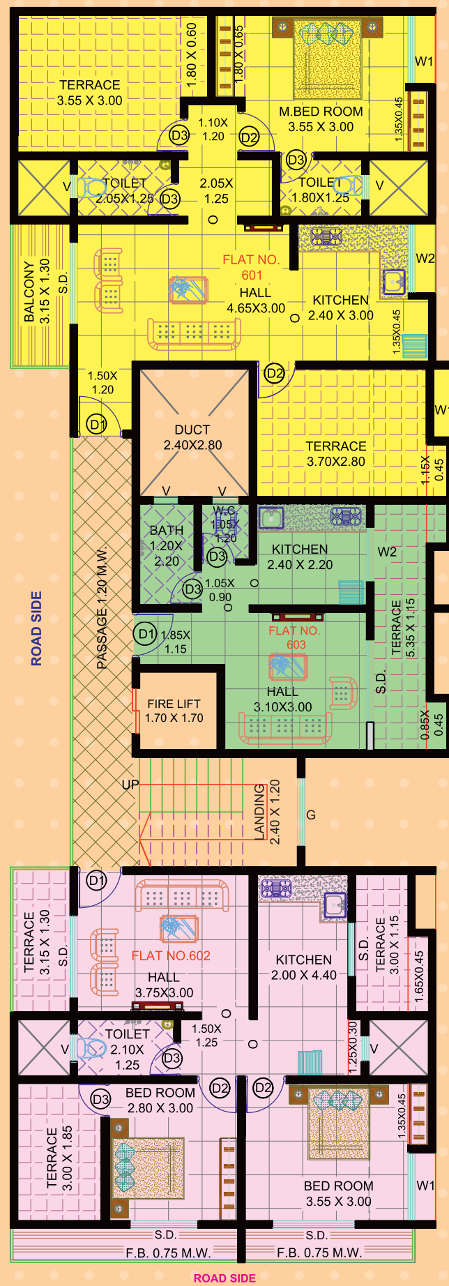
6th Floor Plan
